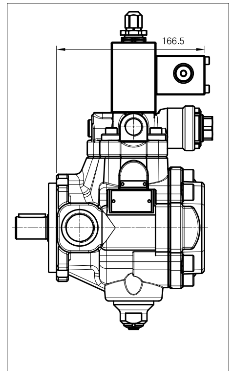
01 PHPK 1-(20-25-32) PCS003 pressure control
